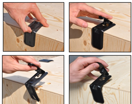
The Clip-Lok QIK Plastic Clips are the easiest & simplest solution available in the market to assemble & disassemble a box.
